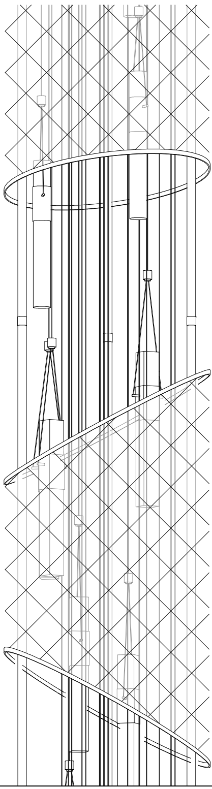
Enlarged details scale: 1"=1'-0"
